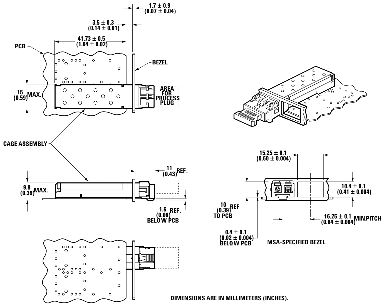
Figure 7c. Assembly drawing
